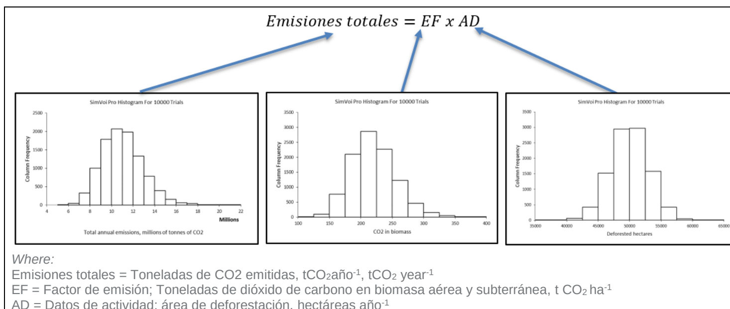
Figure A8. Calculating the distribution of annual emissions from deforestation in one forest stratum
